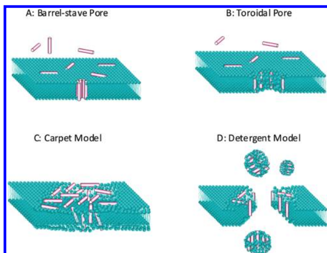
Figure 3. Commonly cited models for antimicrobial peptide activity. Barrel-stave and toroidal pores are membrane-spanning aqueous channels. Antimicrobial peptides are described with the carpet model. Such peptides permeabilize membranes by “carpeting” the bilayer with peptides. At high concentrations carpet model peptides can behave more like detergents.
