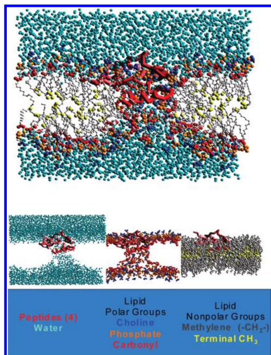
Figure 6. Molecular dynamics simulation of peptide pore formation from Sengupta and Marrink (65). (Top) The peptide-lipid bilayer with CH 2 groups removed. Blue spheres are water molecules, and yellow spheres are the terminal methyl groups. Other color spheres are the lipid polar groups. (Bottom) The same peptide-lipid bilayer separated into groups. Notice that in the vicinity of the peptide “pore” the strict segregation between polar and nonpolar is broken down.
