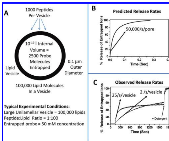
Figure 4. Release of vesicle-entrapped probes. A) A large unilamellar vesicle of 0.1 \mu\text{m} LUV, the type used in most experiments, is made of roughly 10^5 lipids enclosing a volume of about 10^{-19} liter. B) Predicted kinetics of probe release from large unilamellar vesicles containing a single pore of 10 \text{\AA} diameter. Complete release occurs in a few tenths of a second. C) Actual release kinetics observed in experiments with AMPs. Note the difference in x -axis scale indicating that actual release data is 3 orders of magnitude slower than predicted. Furthermore, the simulated release goes to completion, whereas the actual release is incomplete.
