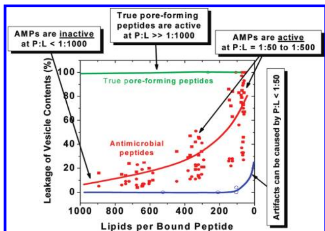
Figure 2. Peptide activity against lipid vesicles. True transmembrane pore-forming peptides, such as alamethicin, permeabilize vesicles at very low peptide to lipid ratios. The green line is based on experimental measurements. Antimicrobial peptides, on the other hand, are active against lipid vesicles only at high peptide to lipid ratios. Data points in red are actual data from several recent publications (13, 17). Almost any peptide that binds to membranes can cause leakage at very high concentration, shown schematically in blue.
